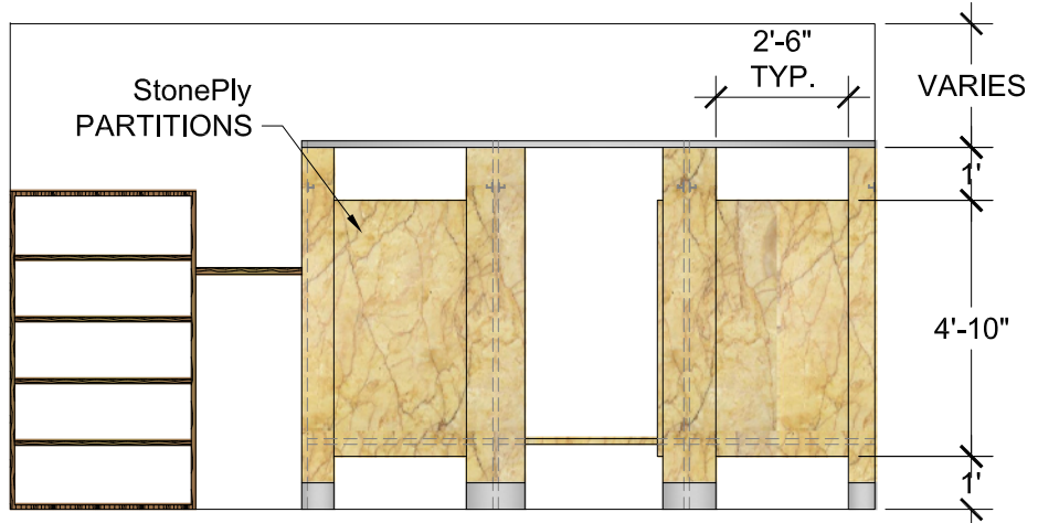
ELEVATION A 1/4" = 1'-0"
