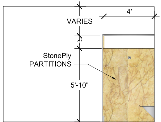
ELEVATION B 1/4" = 1'-0"
