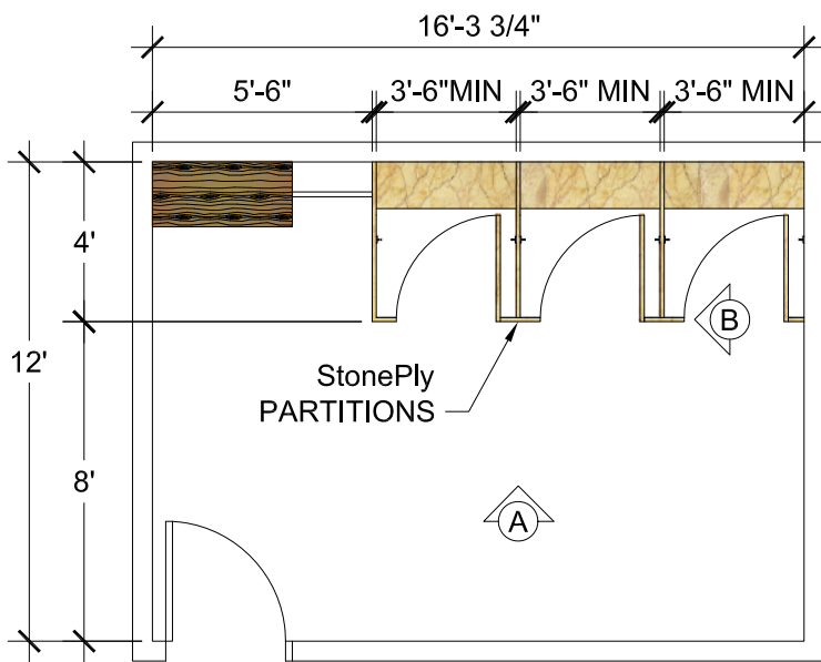
PLAN VIEW 3/16" = 1'-0"
