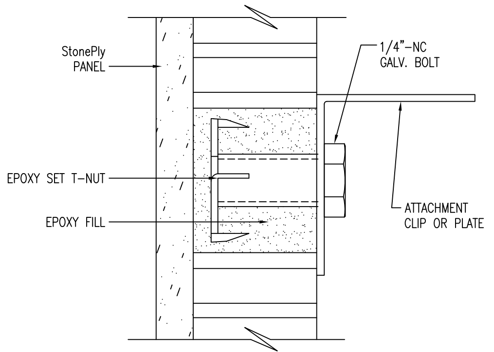
GD1 SECTION DETAIL
