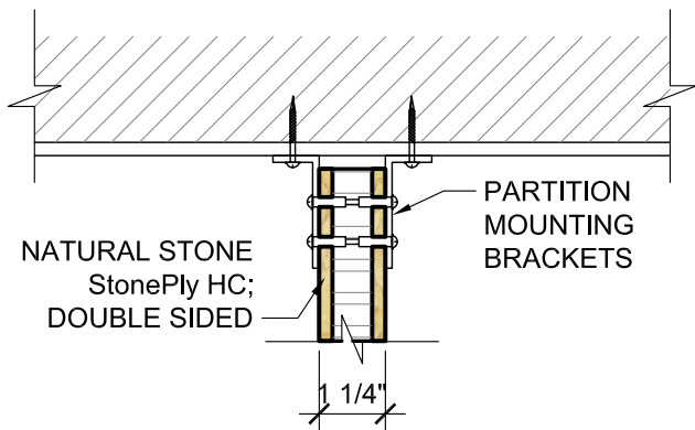
SCREEN MOUNTING DETAIL SCALE: 3" = 1'
