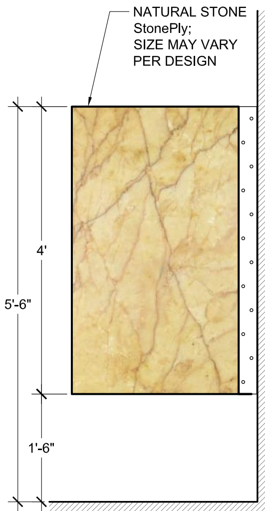
URINAL SCREEN ELEVATION SCALE: 3/4" = 1'
