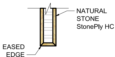
TYPICAL FINISHED PANEL END DETAIL SCALE: 3" = 1'
